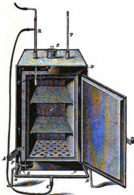
Fig. 38.—Hot-air sterilizer. The gas jets are inclosed within the space between the outer and middle walls, C , and can be seen at F . The heat ascends, warming the air between the two inner walls, which ascends between the walls, K , then descends over the contents, J , and escapes through perforations in the bottom, B , to supply the draft at F , and eventually escapes again at S ; R , gas regulator; T , thermometer.
